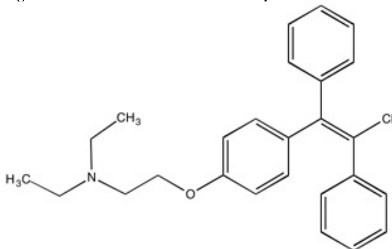
Figure 1. Chemical structure of Enclomiphene Citrate
